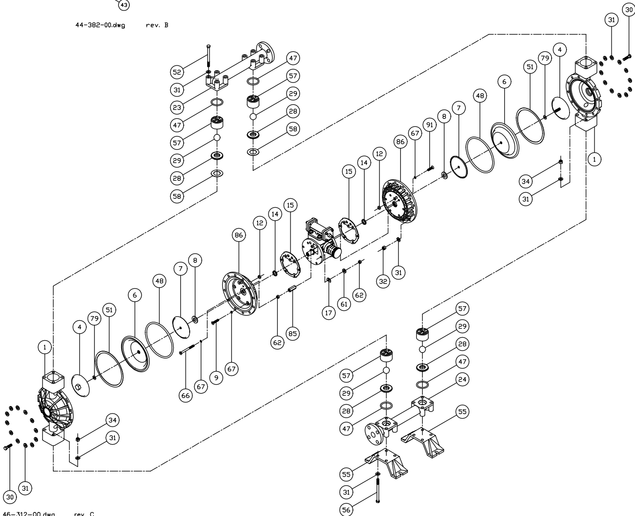
46-312-00.dwg rev. C
